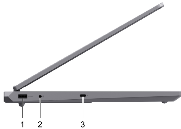
Figure 1. LOQ 15IPH11, LOQ 15IPH11E - Left-side view
