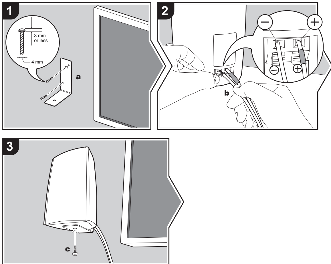
a Wall mount bracket for front speakers, b Speaker cable, c Screw for wall mount bracket (M5×10)
